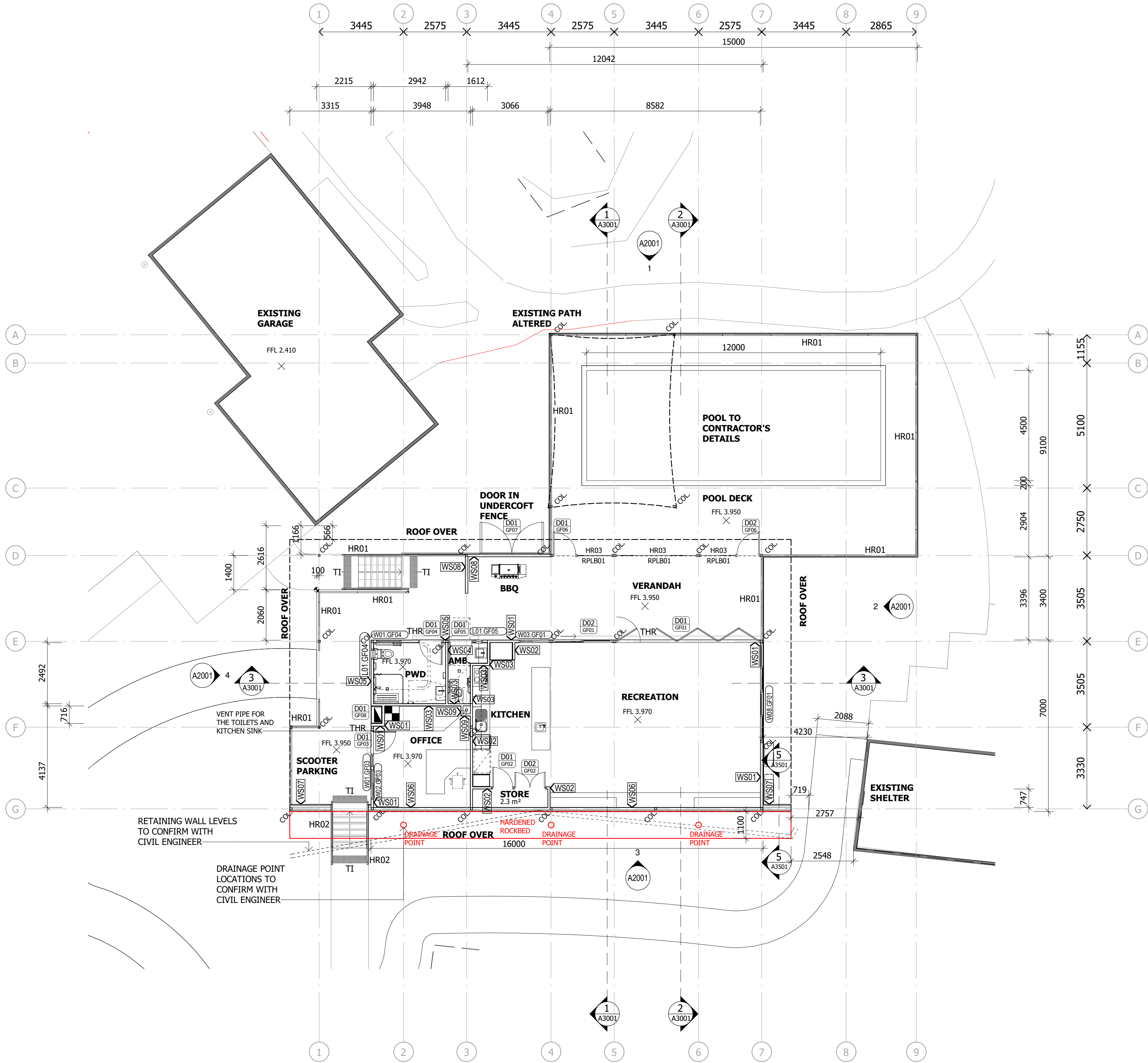
1 GA PLAN - GROUND FLOOR A2001 1 : 100
